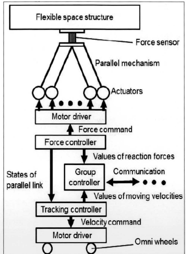
Fig. 16. Structure of Stewart-platform. (Tsujiata, 2014).
