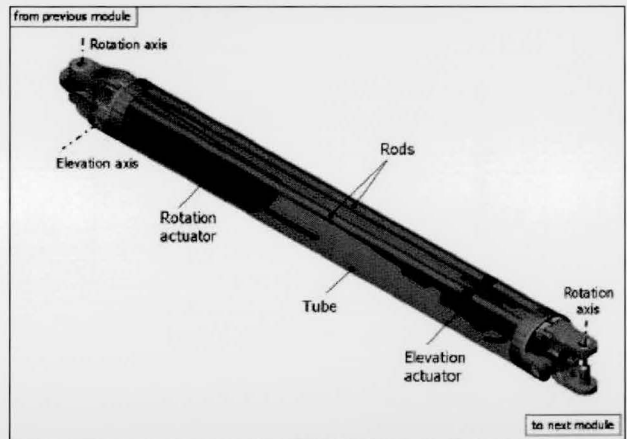
Fig. 8. Remote handling equipment module. (Keller, 2008).
