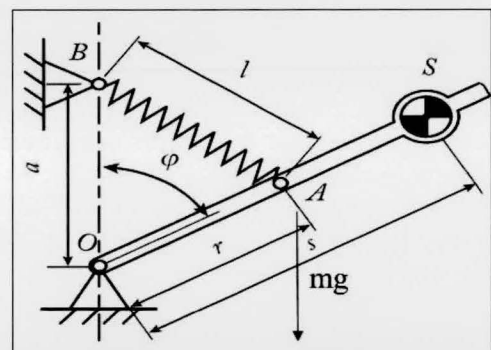
Fig. 3. Gravity compensation by zero free length Spring. (Vigen, 2016).
