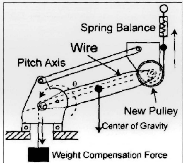
Fig. 11. Counterweight balancing for material handling. (Krüger, 2006).
