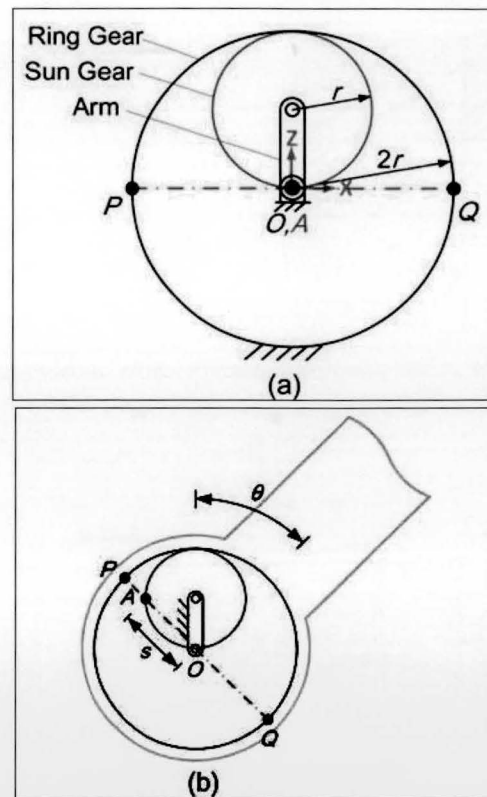
Fig. 7. Cardan gear-based gravity compensation. (Hung, 2017).
