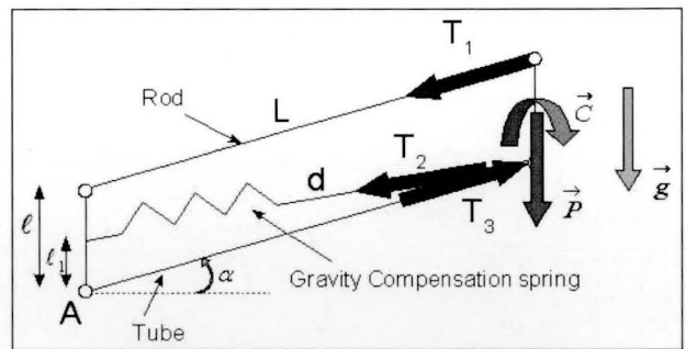
Fig. 9. Gravity forces repartition in the parallelogram structure. (Keller, 2008).
