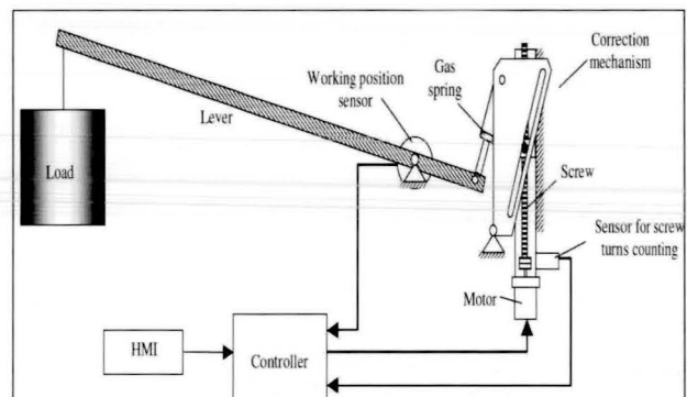
Fig. 12. Lever mechanism with the gas spring and the correction mechanism. (Rogério, 2010).
