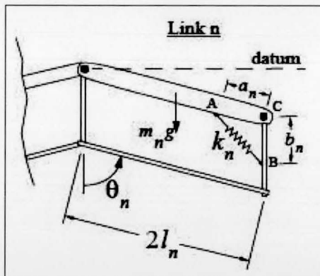
Fig. 5. Gravity compensation by N-links. (Rahman,, 1995).
