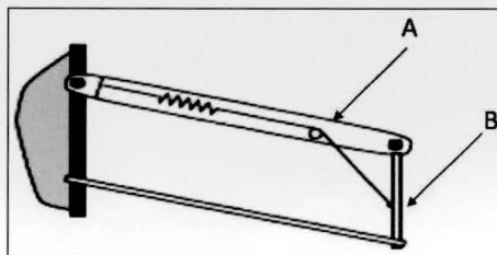
Fig. 6. Gravity compensation by pulley and spring. (Rahman,, 1995).
