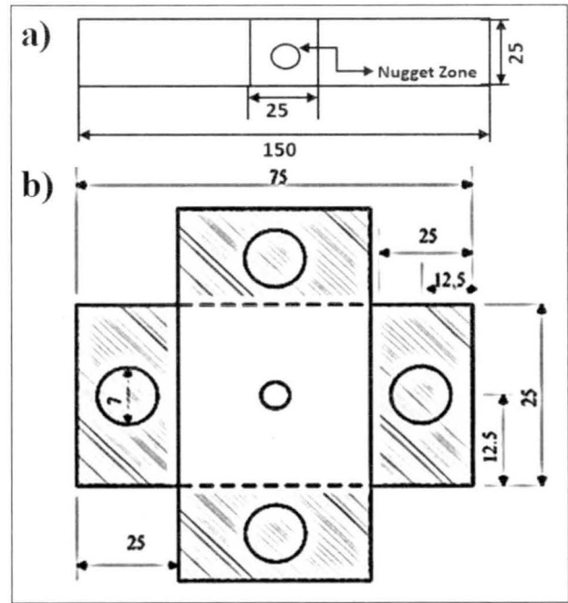
Fig. 1. Dimension of TSFL specimens: a) LAP-TSFL and b) CROSS-TSFL.
