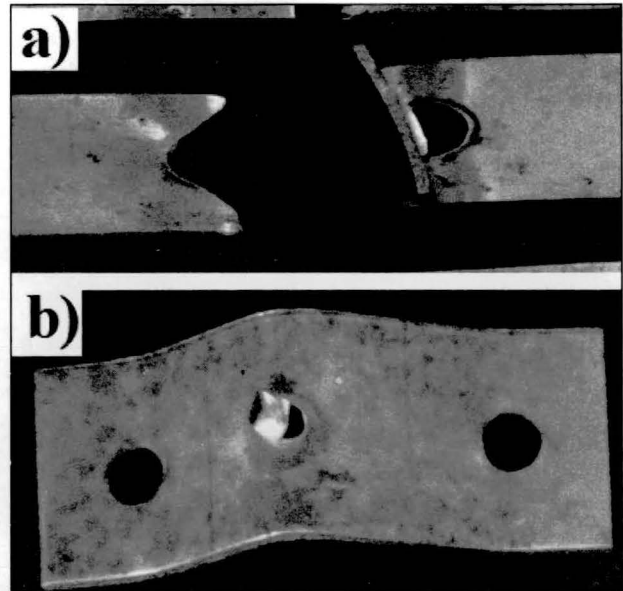
Fig. 4. Failure of optimized joint of RSW DP 800 steel: a) LAP-TSFL and b) CROSS-TSFL specimen.
