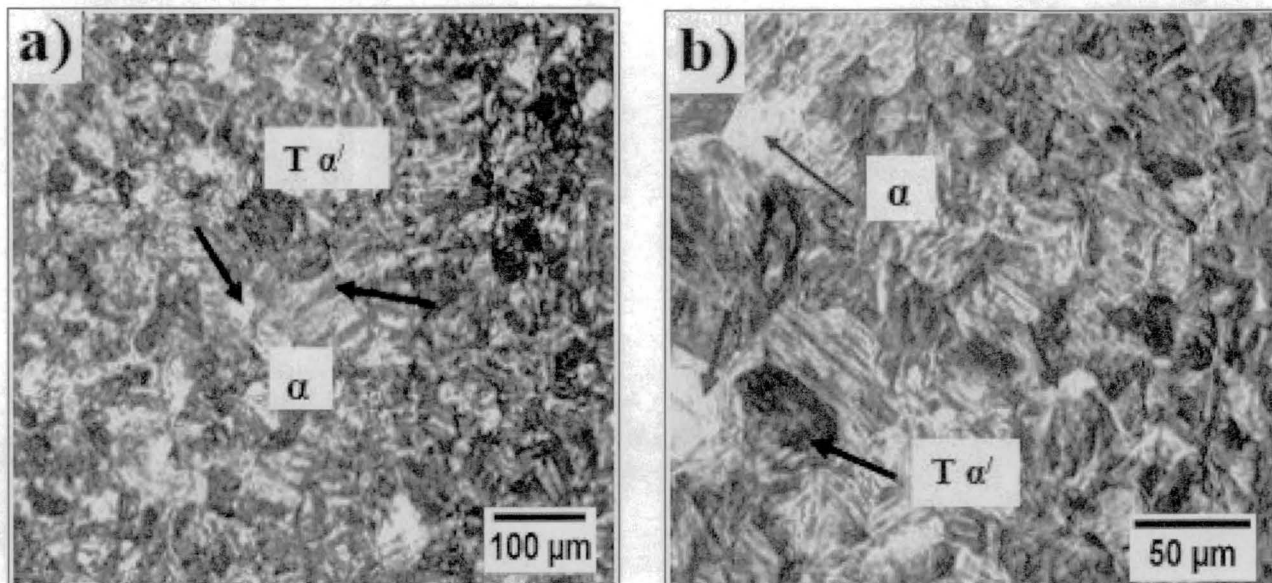
Fig. 10. Optical microstructure of CG-HAZ: a) lower magnification; b) higher magnification.
