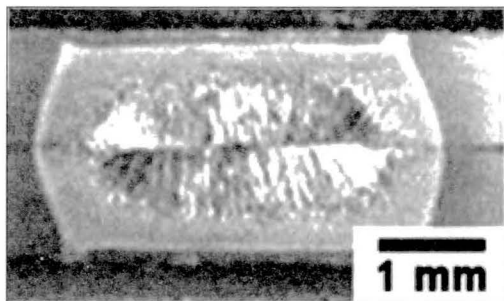
Fig. 8. Macrostructure of AHSS-DP800 RSW joints.
