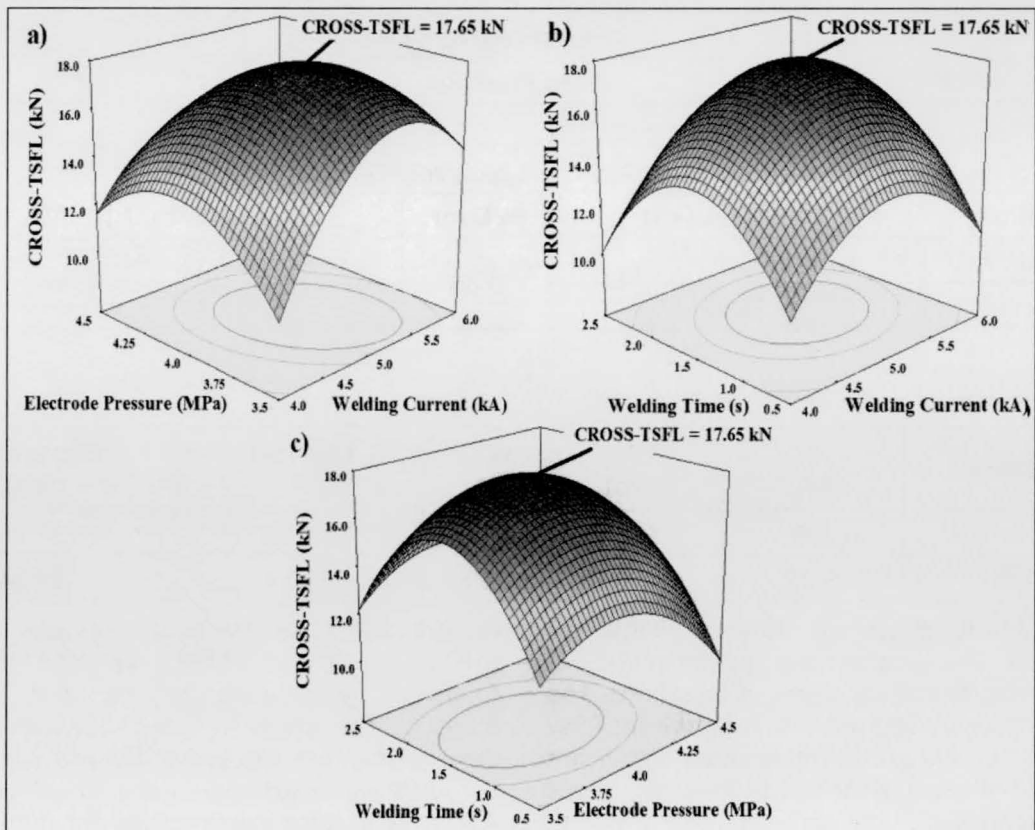
Fig. 6. 3D response surface graphs for CROSS-TSFL.
