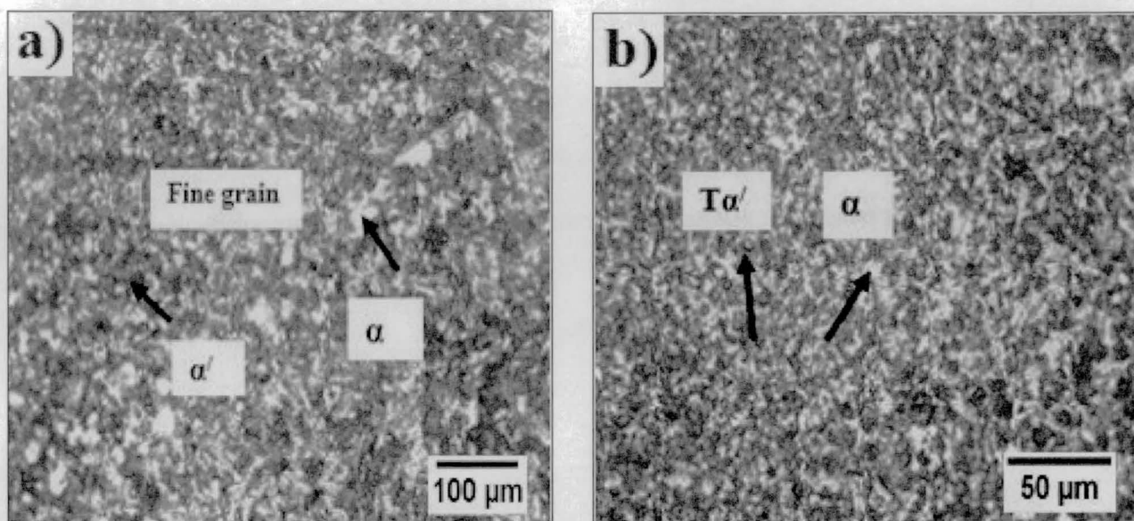
Fig. 11. Optical microstructure of FG-HAZ: a) lower magnification; b) higher magnification.
