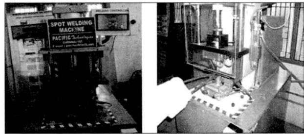
Fig. 2. Photograph of RSW machine.
