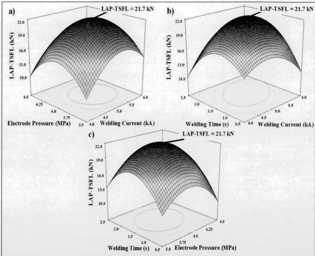
Fig. 5. 3D response surface graphs for LAP-TSFL.
