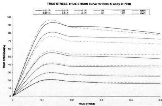
Figure-2: (d) Comparison between the experimental results-R(full lines) & calculated results-C (Dotted lines) by equation (14) at (a) 623K (b) 673K (c) 723K (d) 773K
