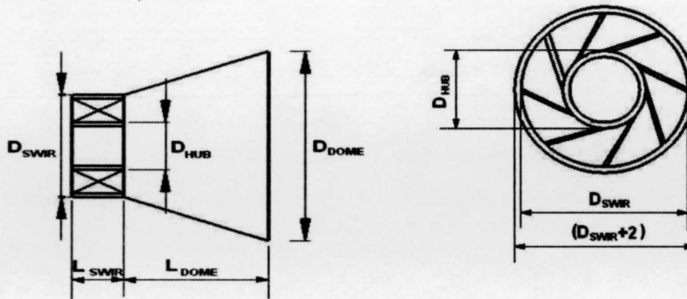
Fig. 1:- Cross-sectional view of SWIRLER
