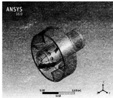
Fig. 2:- Isomeric view of Import geometry in ANSYS at 55°
