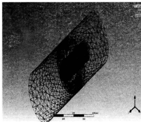
Fig. 3 :- Messing of the SWIRLER geometry
