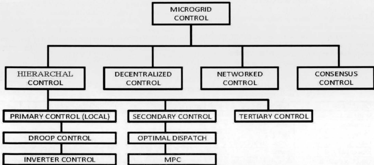
Fig. 6 Microgrid Control
