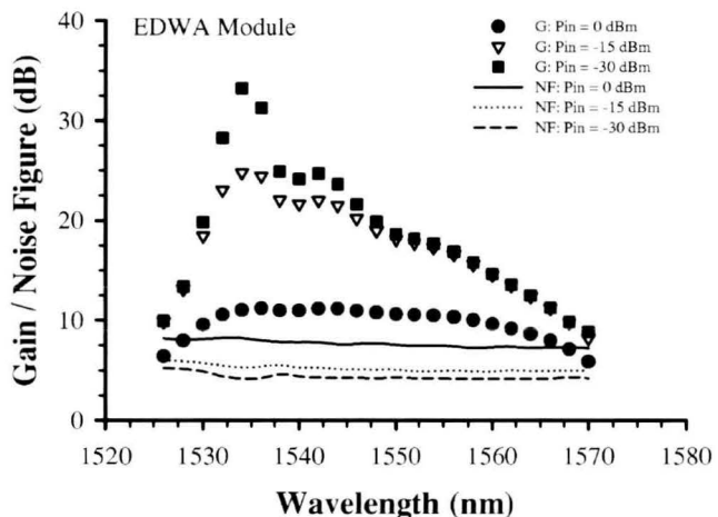
Fig. 3 Gain and noise figure spectra for the EDWA module with the input signal powers P_{in}=0, -15, and -30 dBm, respectively.
