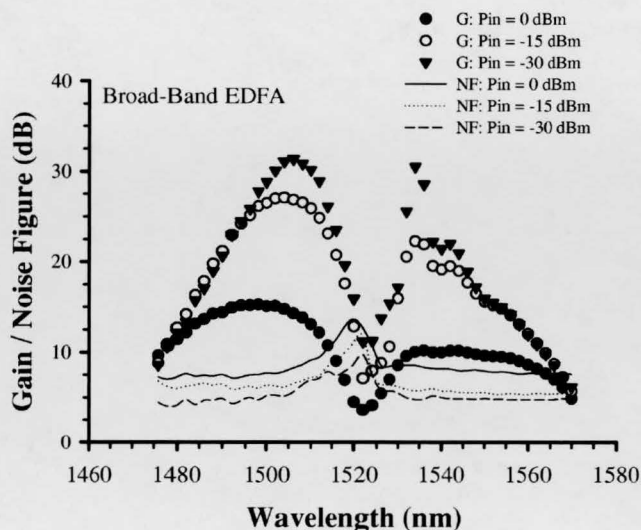
Fig. 5 Gain and noise figure spectra of the proposed configuration with the input signal powers P_{in}=0 , -15 , and -30 dBm, respectively.
