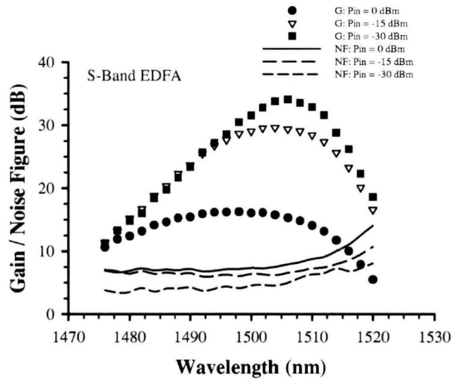
Fig. 2 Gain and noise figure spectra for the S-band EDFA module with the input signal powers P_{in}=0, -15, and -30 dBm, respectively.
