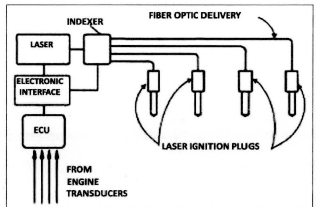
Fig. 5. Working of laser ignition system.
