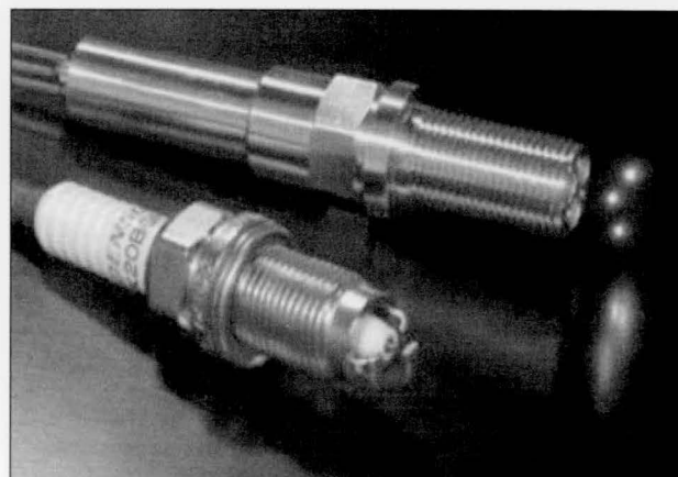
Fig. 7. Electric spark plug & multi-beam laser ignition plug.
