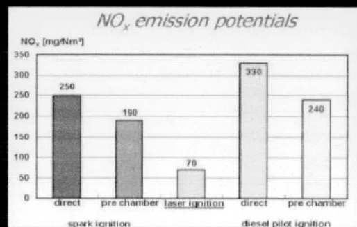
Fig. 8. Bar graph representing NO x emission potentials of different ignition systems.
