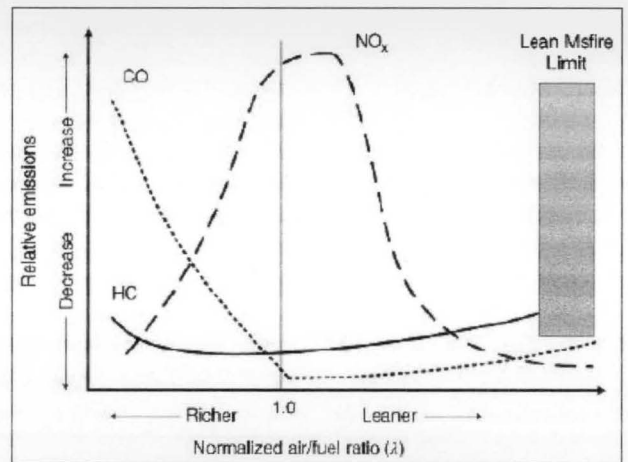
Fig. 2. Graphical representation of emission from engines using an electric spark plug.
