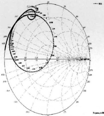
Figure 7: Smith Chart of Single slot arrow shape MSA
